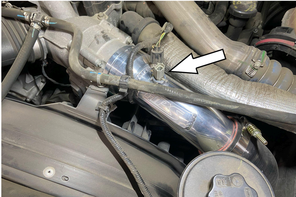
13. Secure the temperature sensor onto the HPS charge pipe and then reconnect the harness.
