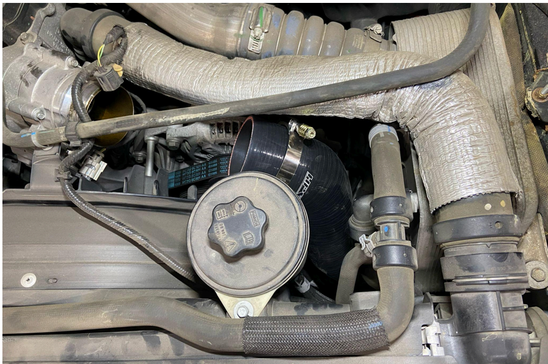
8. Insert the other provided spring loaded T-bolt clamp (83mm-91mm) onto the other end of the HPS charge hose.
