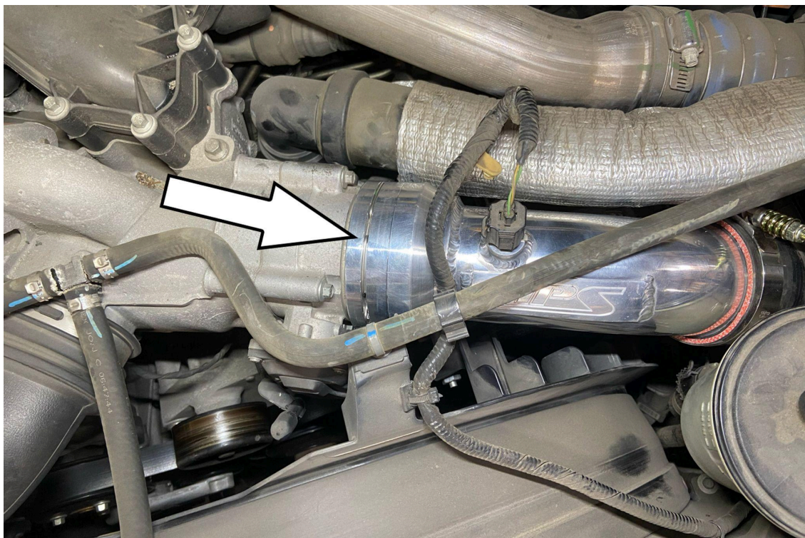
14. Secure the factory retaining clip onto the HPS charge pipe.
