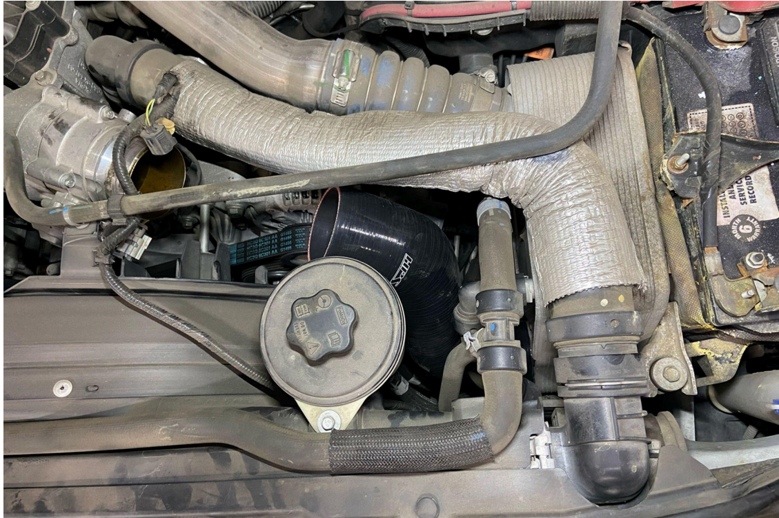
7. Loosely install the HPS charge hose onto the intercooler. Do not tighten the spring loaded T-bolt clamp at this point.
