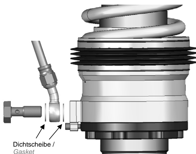
Anschluss Hydraulikleitung / Connecting to the hydraulic line
