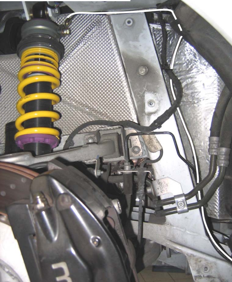
Montageposition 4 / Assembly position 4
