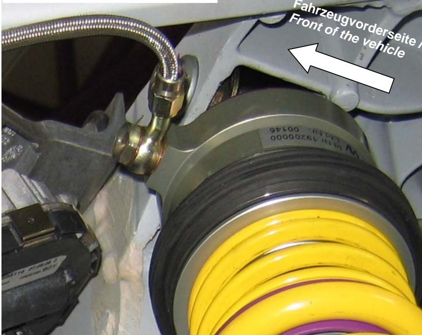
Montageposition 2 / Assembly position 2
