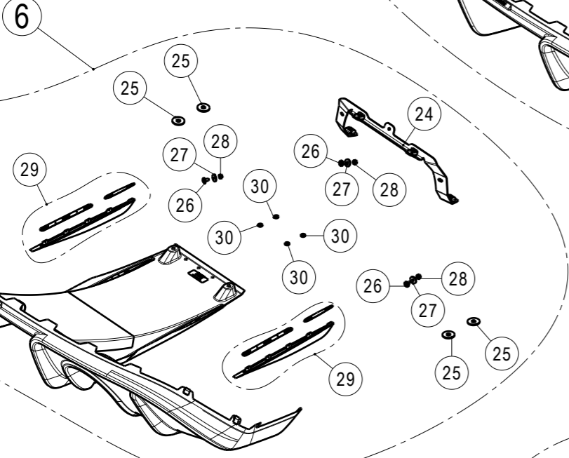
Matte Diffuser 718 Cayman GT4 / Spyder
