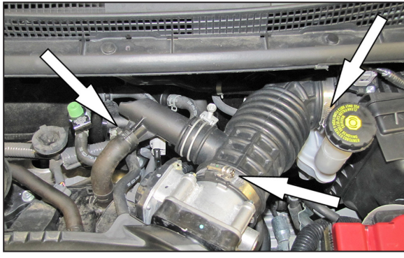
4. Release the spring clamp securing the crank case vent hose to the intake hose and disconnect the hose from the intake tube. Loosen the hose clamps securing the intake hose to the air box and throttle body.
