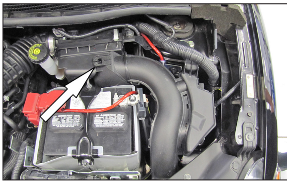
3. Unclip the fresh air intake from the air box and then pull the duct up to unhook it from retaining grommet and remove it from the vehicle.
