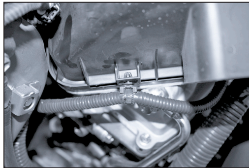
17. Rotate the air box 180° to access the MAF sensor wire harness tie down clip and release it with pliers.
