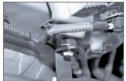
24. Line up Z bracket with the ground mounting bolt from step 23. With provided spacer, washers and bolt secure bracket as shown, make sure to reconnect the ground so that it is underneath the aluminum spacer.
