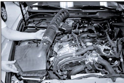
14. Remove the upper air box along with the factory intake tube as shown.
