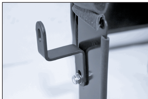
20. Install Z bracket (010033) on heat shield p/n 07340 with provided hardware.
