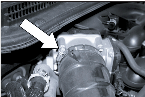
12. Loosen the factory intake tube hose clamp at the throttle body.
