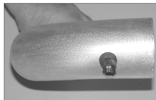
20c. Remove the factory O-ring from the temp sensor then install the sensor into the intake tube as shown.
