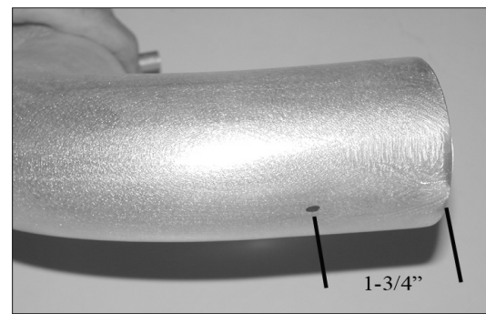
20a. On models that come equipped with an external temp sensor, mark the intake tube 1-3/4" from end of tube, then drill a 3/4" hole into intake tube.
