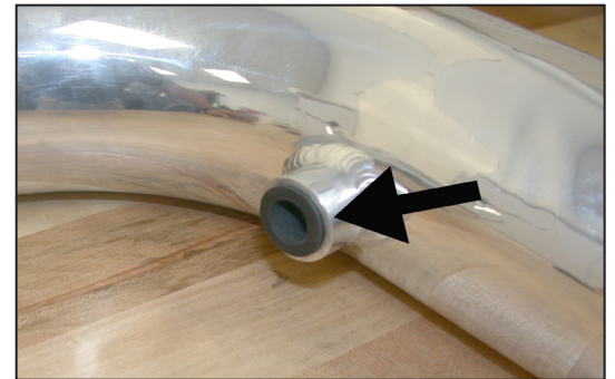
24. Install the provided silicone hose into the vent on the K&N® intake tube as shown.
