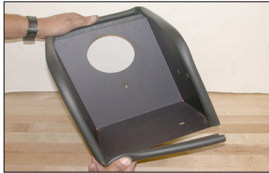
17. Install the provided edge trim onto the heat shield as shown.
