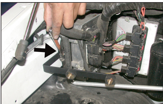
14. Secure the "L" bracket assembly to the threaded hole from step 12 using the original bolt as shown.
