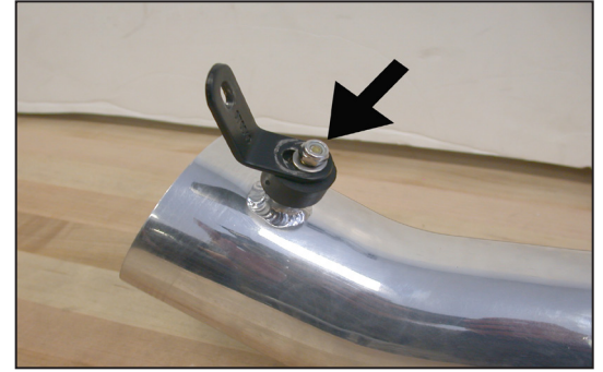
23. Install the angled bracket onto the rubber mounted stud using the provided hardware as shown, but do not tighten completely at this time.
