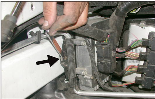
12. Remove the screw that secures the computer to the inner fender as shown.
