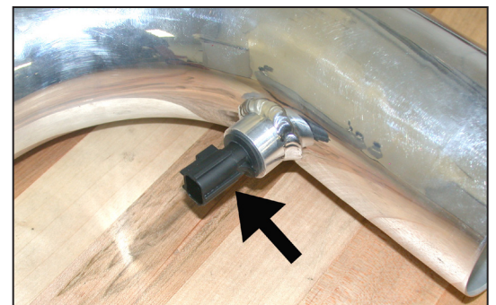
25. Slide the air temperature sensor into the silicone hose as shown. NOTE: The plastic cage on the end of the air temperature sensor is very fragile so take care when installing the air temperature sensor into the silicone hose.
