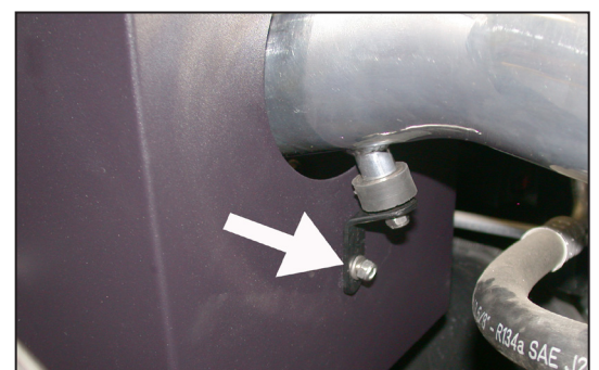
27. Secure the angle bracket to the heat shield using the provided hardware as shown, but do not tighten completely at this time.
