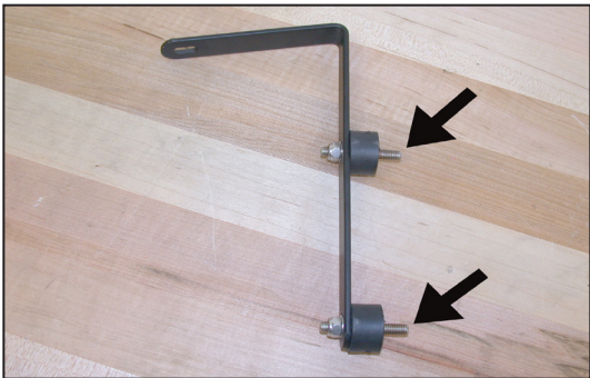
13. Install the rubber mounted studs onto the "L" bracket using the provided hardware but do not completely tighten at this time.
