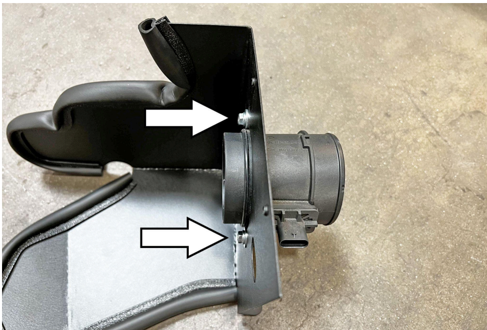
10. Secure the mass air flow sensor housing onto the lower HPS heat shield using the provided M6x16mm bolts (2), nuts (2), and washers (4).
