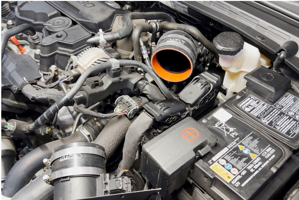
16. Install the couplers onto the turbo inlet and mass airflow sensor housing using the provided EMSC clamps.
