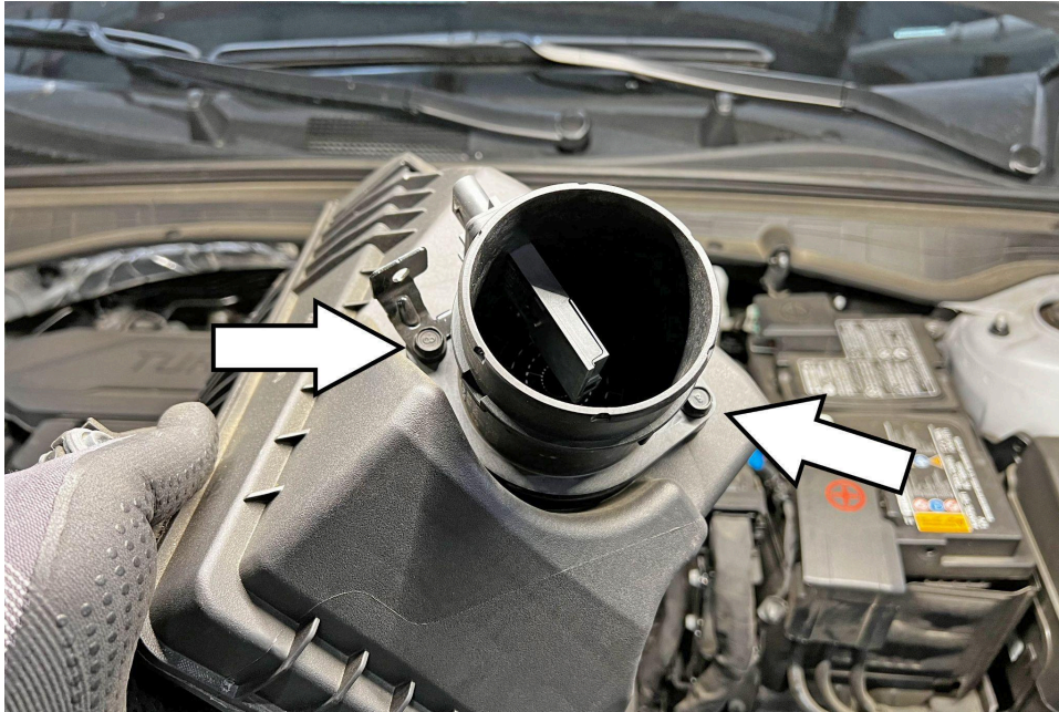
9. Loosen the two 10mm bolts to remove the factory mass air flow sensor housing from the air box assembly.
