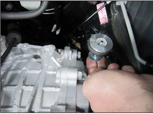
f. From underneath the factory rubber grommets, slide each bolt and fender washer through so the bolt protrudes through the rubber grommet and adapter as shown.
