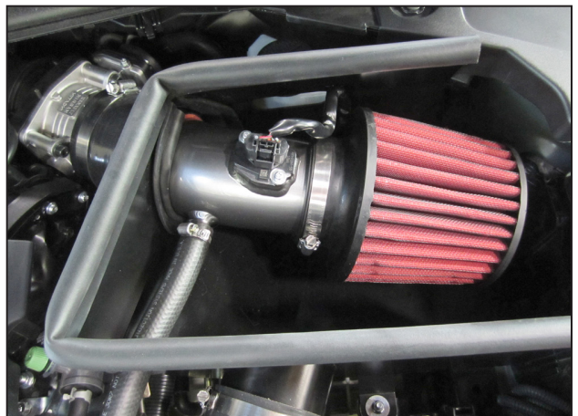
ai. Attach the PCV vent hose to the intake pipe's vent. Secure the vent hose with hose clamp (08411) and connect the MAF sensor harness plug to the MAF sensor.
