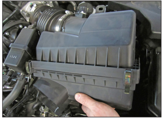
l. Lift up on the bottom of the air box to disengage but do not remove from engine bay.
