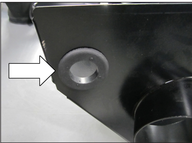
j. Insert the rubber grommet (784640) into the heat shield hole as shown.
