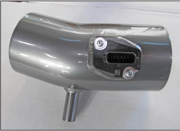
ad. Install the MAF sensor onto the intake tube (2-1481) using the OEM screws.
