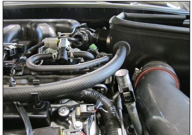
ac. Feed the PCV vent hose through the heat shield hole as shown.
