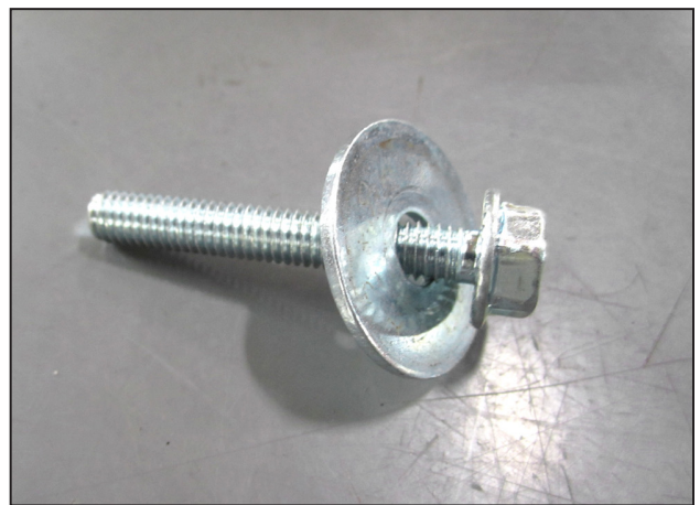
e. Slide a fender washer (08160) onto each of the M6x35mm bolts (1-2002 ) as shown.
