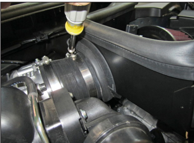
ah. Align the intake pipe with the throttle body's coupler and secure the #52 hose clamp.
