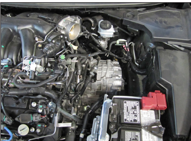
o. Remove the factory air box system from the vehicle.
