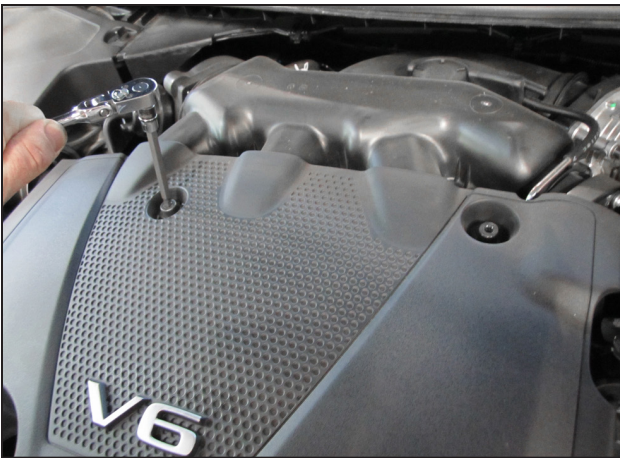
a. Remove the two 5mm Allen head bolts that secure the valve cover in place.
