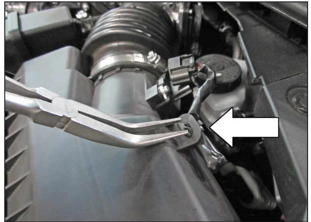
h. Release the clip securing the MAF sensor harness to the air box.
