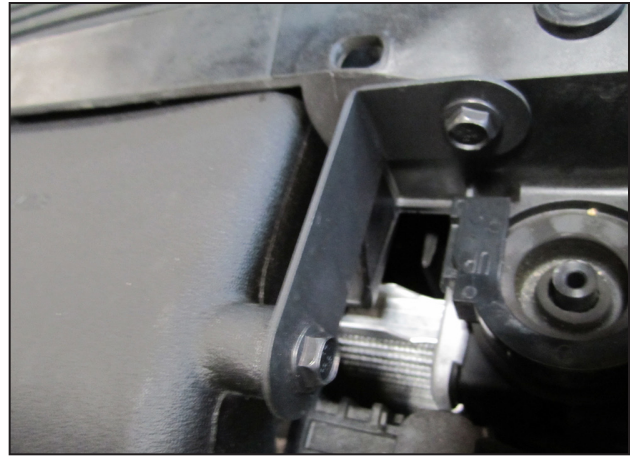
y. Secure the air inlet scoop's bracket to the radiator support using one M6 bolt (1-2110).
