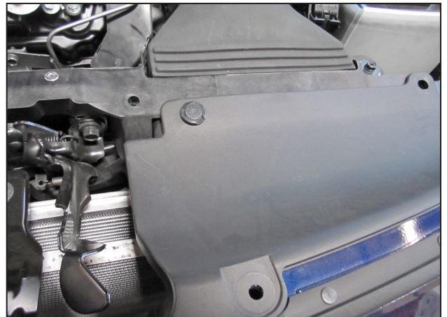
ao. Install the 8 clips to secure the radiator shroud, beginning with the clip securing the air inlet scoop in place.
