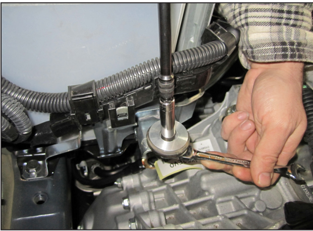
h. Once properly assembled, tighten the nuts and bolts to secure the adapter assemblies.
