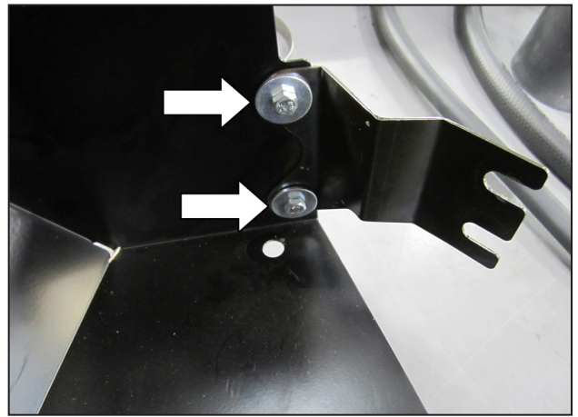
i. Attach the provided bracket (7-7885) onto the heat shield using 2 M6 bolts (1-2065) and 2 washers (08160).
