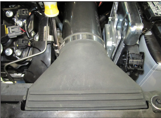
al. Tighten the hose clamp securing the air inlet hose to the air intake tube.
