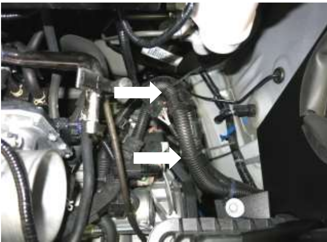
g. Using the two supplied zip ties, bundle wiring harnesses as shown in these locations. Clip excess zip tie lengths with diagonal cutters.
