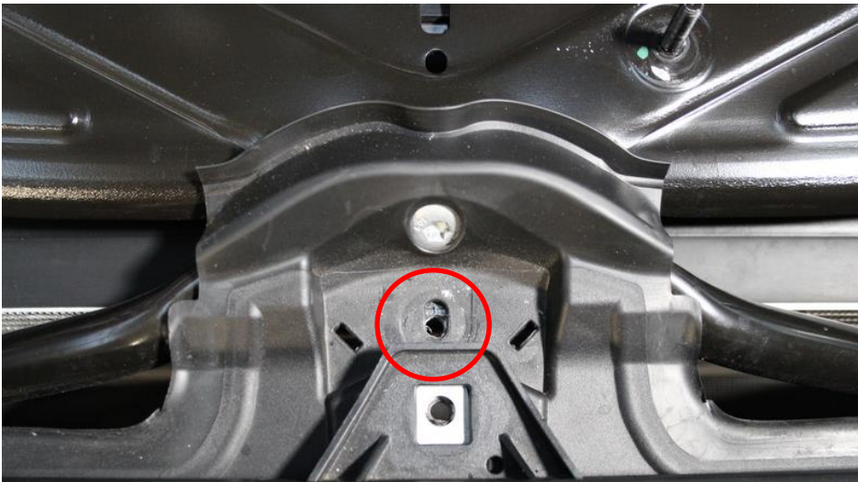
11. Now remove the middle Torx screw which is partially under the plastic tab of the bumper.
