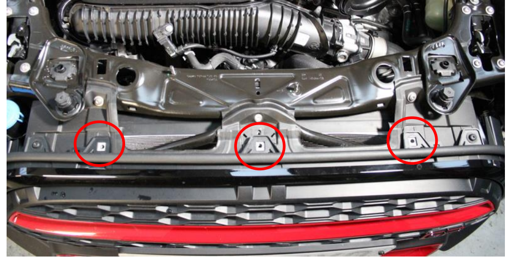
10. First remove the 3 Torx screws which secure the top of the front bumper.
