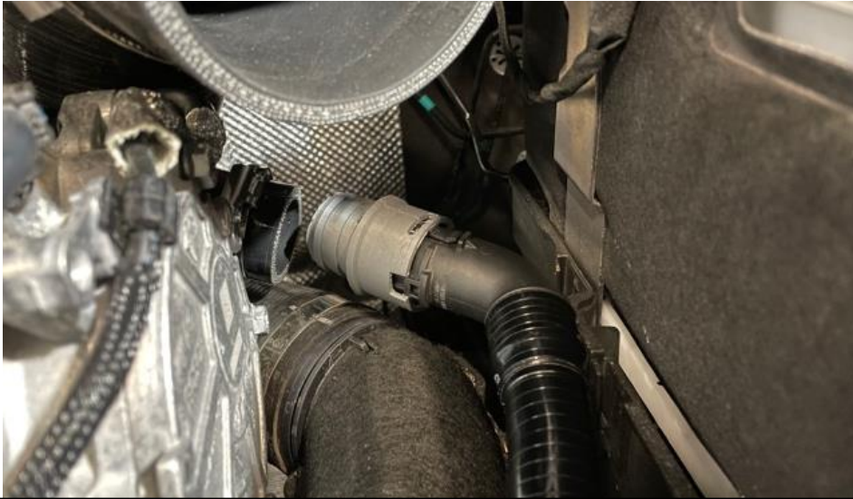
13. Now push the fitment into the silicon hose (Golf R only).
