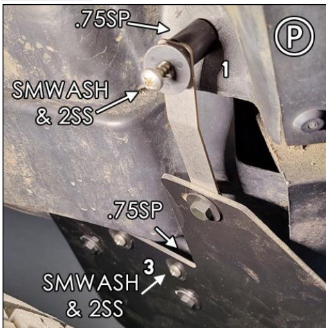
FIGURE Q/R Ensure flap is aligned to vehicle before tightening fasteners.
