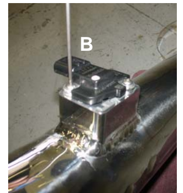
Figure 18 A) Align bracket to vibra mount and secure. B) With provided fender washer and M6 nut secure bracket. Do not tighten.
