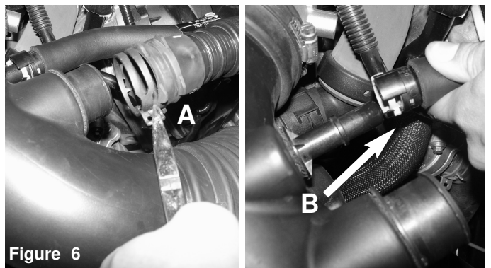
Figure 6 A) With pliers loosen the clamp holding in the sound tube connected at the intake tube and remove. Pull back sound tube. B) Disconnect crank case line from intake tube.
