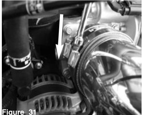
Figure 31 Now tighten the clamps on throttle body using 8mm nut driver.
