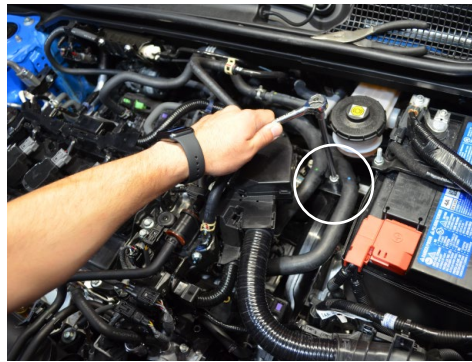
14. Remove the bolt securing the coolant line bracket.
