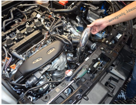
38. Install the hot side intercooler pipe. Insert the pipe into the bottom hose then into the top step hose.
