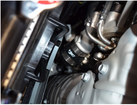
37. Install the 1.875"-2.25" hose onto the turbo. Only secure the clamp on the turbo.
