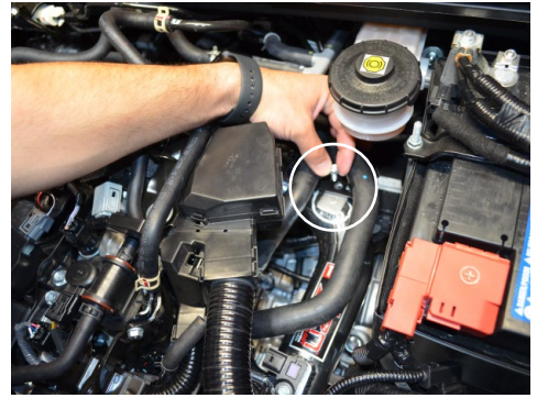
27. Secure the coolant line bracket with the provided M6 bolt.
