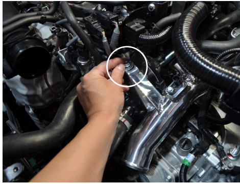
26. Secure the intercooler pipe bracket to the throttle body hose with the provided M6 nut and washer.
