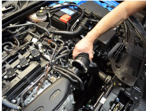
5. Loosen the clamp securing the intake tube to the turbo inlet then detach the tube.
