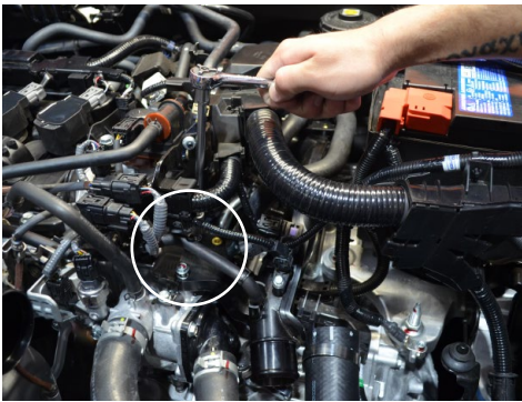
13. Remove the two bolts securing the intercooler pipe bracket to the engine.
