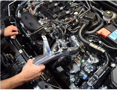
25. Install the primary cold side intercooler pipe to the throttle body hose. Leave the clamp loose for now.
