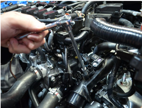
16. Disconnect the pressure and temp sensor harness, then remove the bolts securing the sensors.
