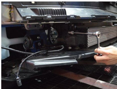
35. Secure the intercooler adapter to the inlet on the intercooler using the the OEM bolts.
