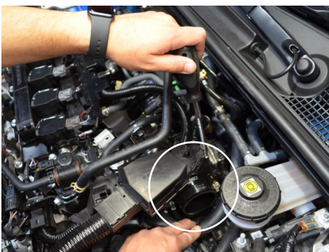
22. Install the 2.50" hump hose onto the throttle body. Only secure the throttle body clamp.
