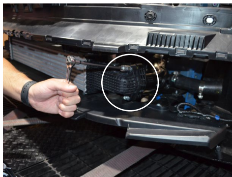
11. Remove the two bolts securing the cold side intercooler pipe to the intercooler.
