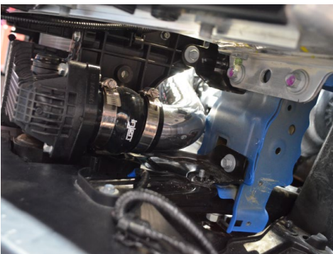
34. Adjust both tubes for best fitment then secure all remaining clamps.
