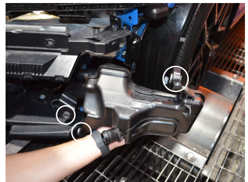
9. Remove the three bolts securing the intercooler pipe resonator, then remove the resonator.
