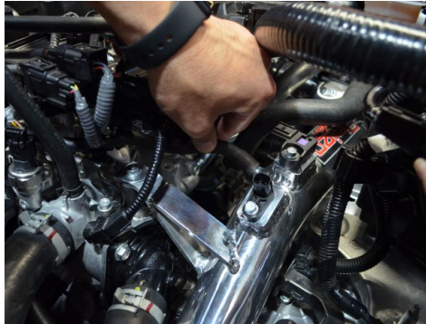
29. Reconnect the vacuum line to the vacuum fitting on the intercooler pipe.
