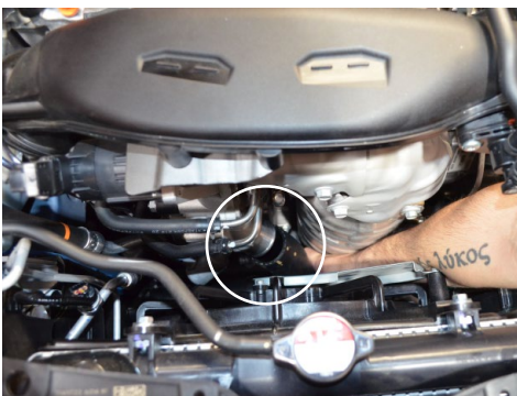
19. Loosen the clamp securing the hot side intercooler pipe to the turbo, then detach the pipe.
