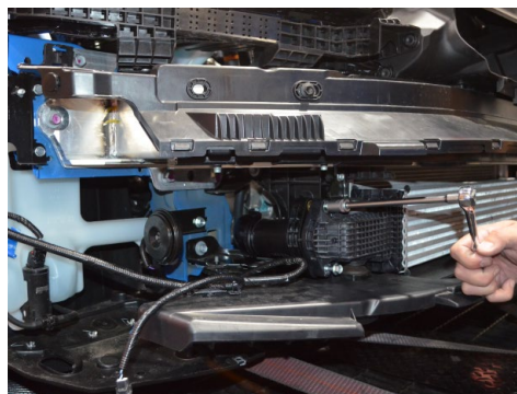
20. Remove the two bolts securing the intercooler pipe to the intercooler.
