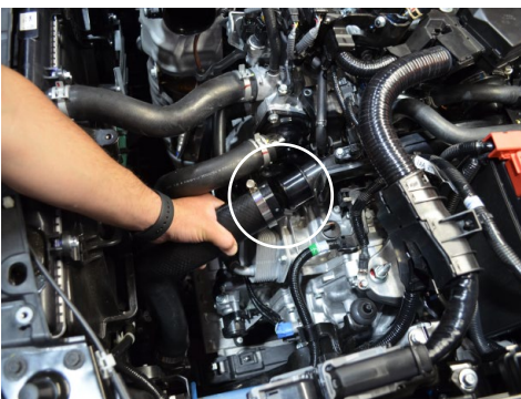
10. Loosen the clamp securing the rubber intercooler hose to the top half of the cold side intercooler pipe, then detach the hose.
