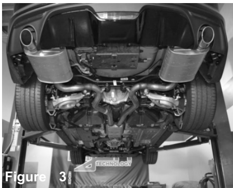
OEM exhaust system. Secure vehicle on lift.
