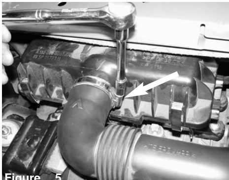
Figure 5 Loosen the clamp on the stock air box.
