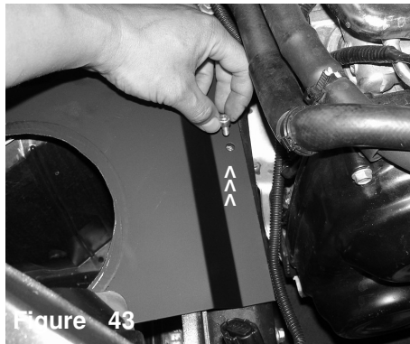
Figure 43 The heat shield bolt hole on the step side is lined up to the pre-tapped hole in the frame. Use the m6 x 12mm bolt in the kit to secure the heat shield.
