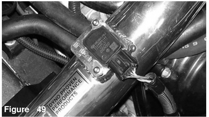
Figure 49 The electrical harness is firmly connected on the mass air flow sensor.
