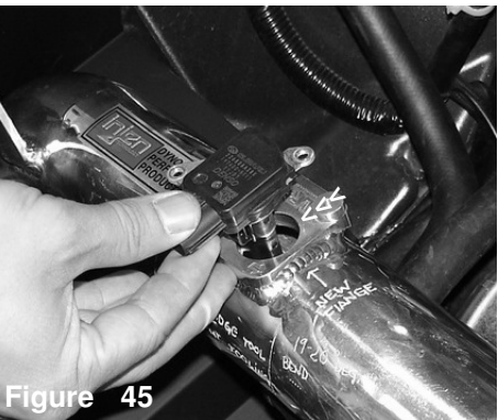
Figure 45 The mass air flow sensor is carefully inserted into the machined sensor flange. Use a dab of light oil around the O-ring to prevent it from kinking or tearing.
