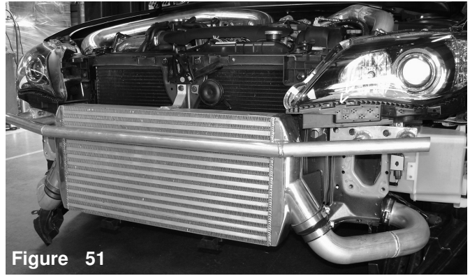
Figure 51 Coming soon, the SES1204FMGT- Large front mount intercooler with a replacement bumper support and intercooler piping.
