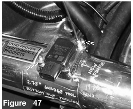
Figure 47 An allen wrench is used to tighten the stock screws on the mass air flow sensor.
