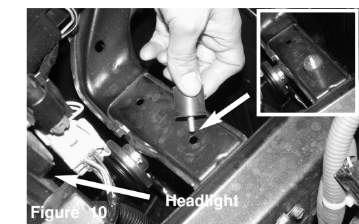
Figure 10 Locate the hole on the chassis support bracket behind the passenger side headlight. Mount the supplied vibramount to this hole and place a M6 nut from underneath and secure the vibramount to the bracket
