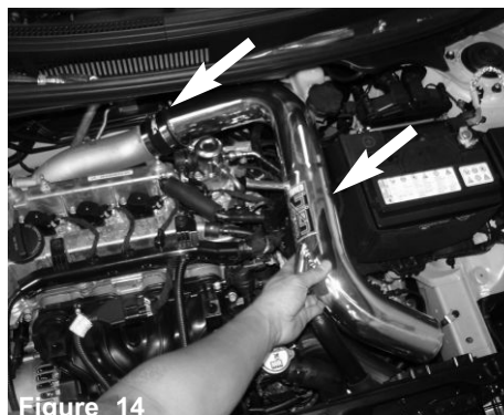
Figure 14 Position the intake pipe into the engine bay and place the end of the pipe into the step hose on the turbo compressor outlet.
