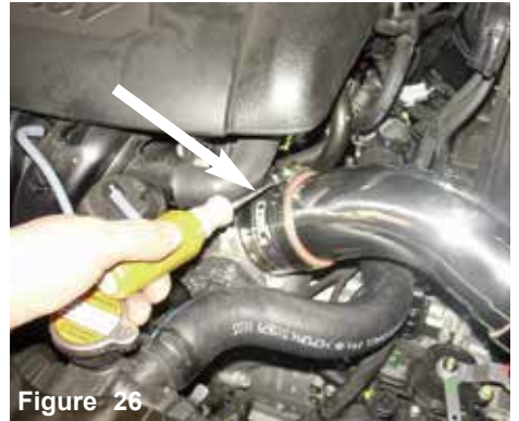
Figure 26 Position for best fit and tighten the remaining clamp on the throttle body using 8mm nut driver.
