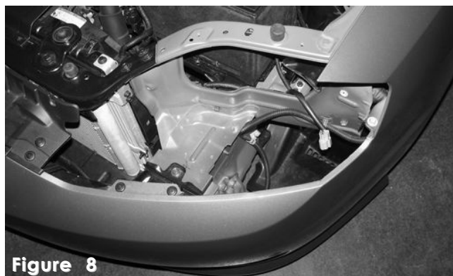
The head lamp is now removed
