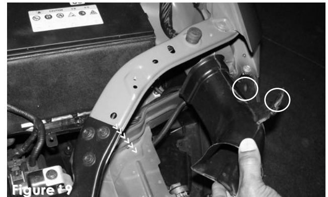
Remove plastic clips or bolts from the air intake duct connected to the fender well. Once fasteners have been removed, continue to remove the plastic air duct from the fender well.
