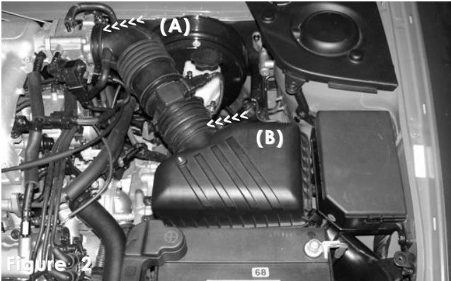
Loosen clamp on the throttle body (A) and air intake duct with mass air flow sensor (B).
