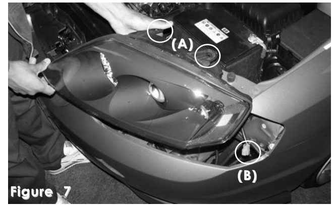
Remove two bolts located on the head lamp frame (A). Disconnect harness clip from the rear head lamp and remove harness clip (B). Once bolts and clips have been removed, continue to remove head lamp as shown above.
