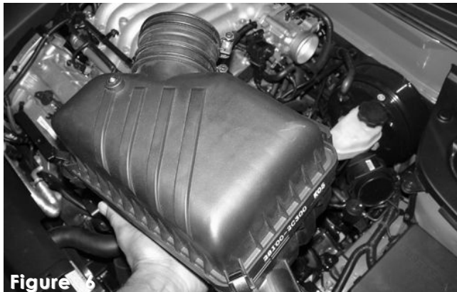
Once you have removed the three bolts from the lower air box, continue to remove the entire air box cleaner.
