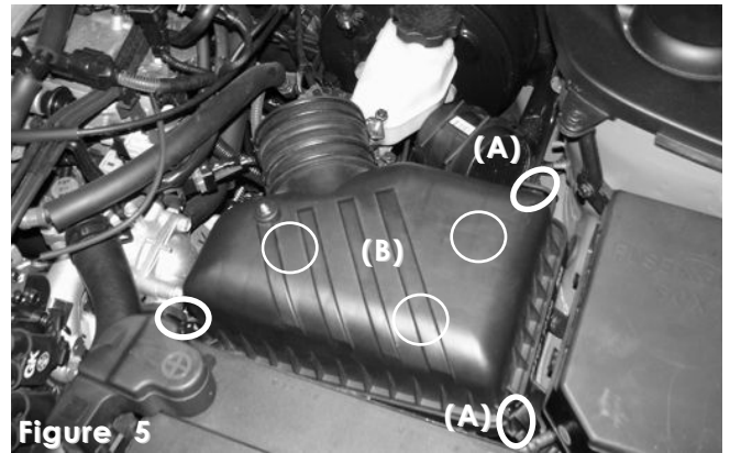
Remove the three clips that secures the top cover to the bottom air box (A). Separate the top cover from the lower air box, then remove the panel filter. Now remove the three bolts that holds the lower air box to the brace (B).
