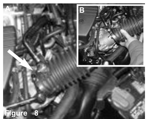
Figure 8 Figure A: Use a 10mm socket and ratchet to loosen the clamp on the rubber air duct connected to the throttle body. Figure B: Pull the rubber duct off the throttle body
