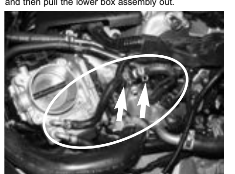
Figure 14 Now connect the other coolant line from the upper radiator hose housing to the coolant line hose from the throttle body.
