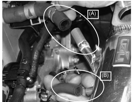
Place the intake into the engine compartment and locate the crank case breather hose (A) and the air control thermal vacuum hose (B).
