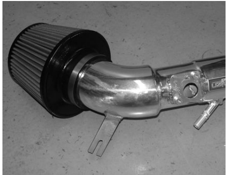
Once the filter has been properly placed over the intake end, continue to tighten the filter neck clamp.
