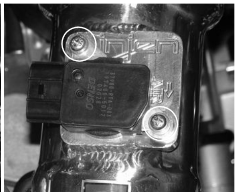
The sensor is in place and the stock screws have been reused to secure the sensor to the adapter.
