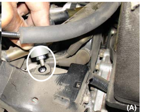
Once the 6mm bolt has been removed screw the vibra-mount into its place (A). Make sure that the vibra-mount is completely screwed into the pre-tapped hole (B).
