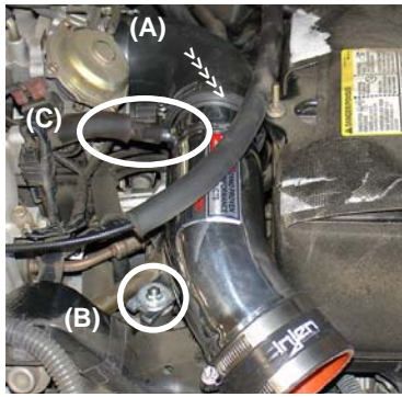
Once the intake has been pressed into the elbow on the throttle body (A) Align the intake bracket to the vibra-mount stud (B). Press the stock vacuum line over the intake port (C).
