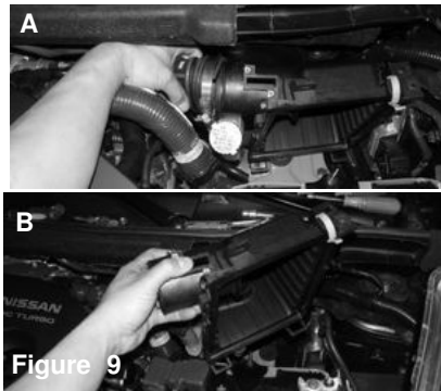
Figure 9 Figure A: Detach the air duct hose from the air box housing. Figure B: Remove the entire rear air box housing
