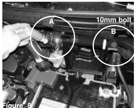
Figure 8 Figure A: Use an 8mm nut driver and loosen clamp on air duct to air box. Figure B: Loosen 10mm bolt on air box attached to bracket on shock tower.
