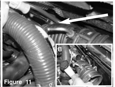
Figure 11 Figure A: With 8mm nut driver, loosen the clamp on the turbo. Figure B: Remove the stock turbo auxiliary hose.
