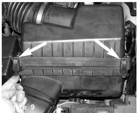
Figure 9 Unlatch the two metal clips shown above.
