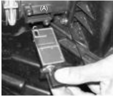
Remove the two screws from the sensor pad (A) and carefully remove the air sensor from the sensor housing as shown above.
