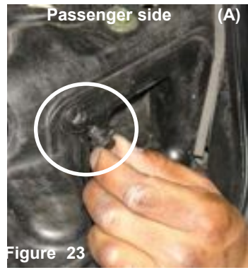
Figure 23 Remove the plastic clips from the front air scoops which are located in front of the passenger side (A) and the driver side (B) cross member.
