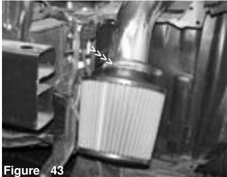
Figure 43 Once the intake end is butted up to the filter stops, continue to tighten the filter clamp.
