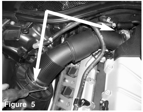
Figure 5 Loosen the clamp on the throttle body and air box side using 7mm nut driver.
