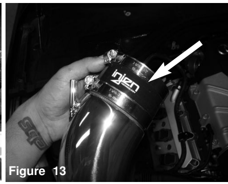
Figure 13 Attach the 3" hose with clamps provided to the intake tube. Do not tighten.
