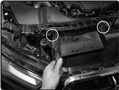
4. Locate the 2 bolts holding in the front air scoop and loosen and remove using T25 torx bit.
