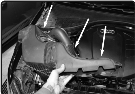
8. Carefully lift up and remove the entire air box assembly out of vehicle.
