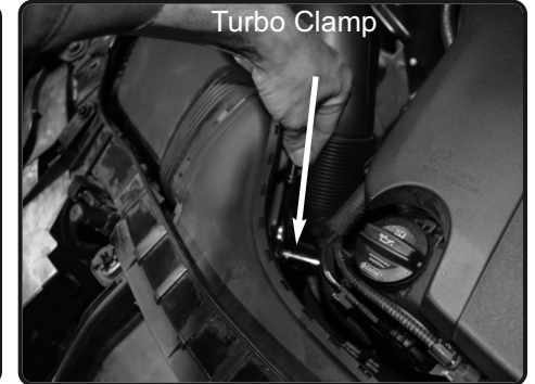
7. Loosen the clamp on the turbo using 7mm socket with ratchet.
