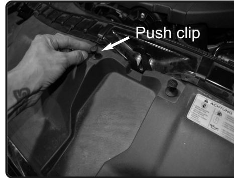
7. Carefully remove the push clips using flat head or panel clip removal tool.
