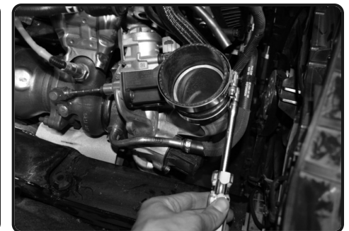
11. Tighten the clamp on turbo only.
