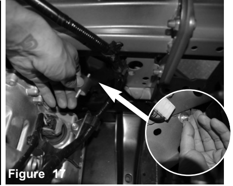
Figure 17 From the inside of the engine compartment, locate the hole from the previous step, and secure from the other side using provided M6 nut and fender washer.
