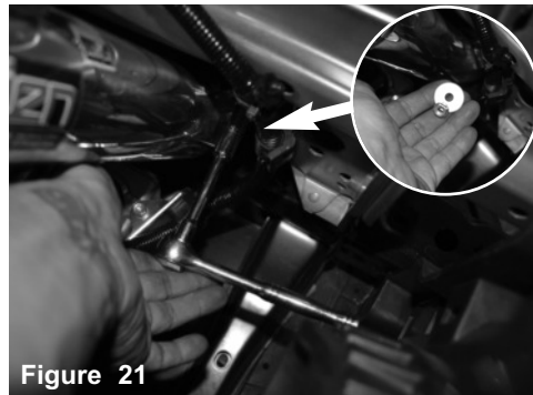
Figure 21 Secure the bracket to the vibramount using provided m6 nut and fender washer. Do not tighten.
