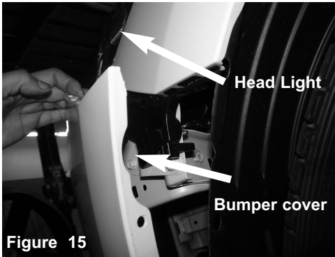
Figure 15 Loosen the screws and pull back the bumper cover on driver side, this will allow filter installation. Loosen the screws on side and bottom of the splash guard also. This will allow for filter installation.
