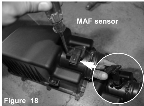
Figure 18 With Phillips screwdriver, loosen the 2 screws holding in the MAF sensor. Remove the MAF sensor from the stock intake tube.
