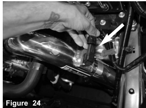
Figure 24 Re-connect MAF sensor harness.
