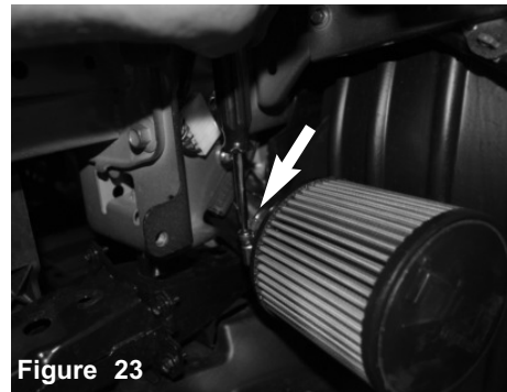
Figure 23 Install the air filter and tighten using 8mm nut driver.
