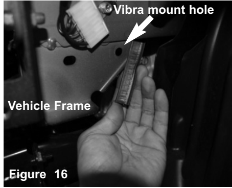
Figure 16 With provided trim-seal, attach to the lip that is on the vehicle frame. This will prevent any contact with the intake and frame. Take note of hole that will be used for the vibramount.
