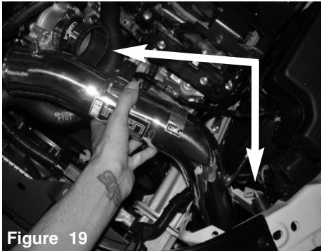
Figure 19 Install the intake tube and position the bracket to the vibra mount and to the throttle body.
