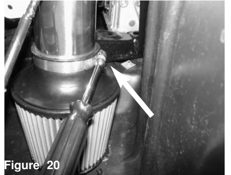
Figure 20 Now attach air filter to the intake tube and tighten using 8mm nut driver.
