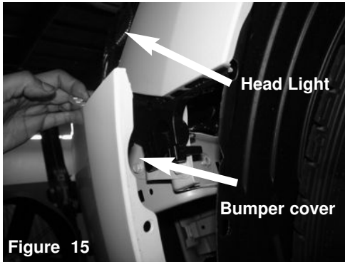
Figure 15 Loosen the screws and pull back the bumper cover on driver side, this will allow filter installation. Loosen the screws on side and bottom of the splash guard also.
