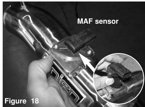
Figure 18 Install the MAF sensor into the intake tube and secure using provided M4 screws. Tighten using 2.5mm allen key.
