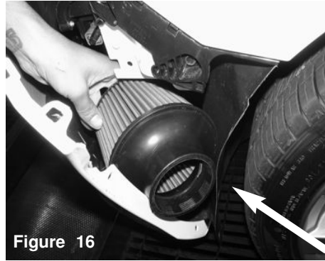
Figure 16 Now install filter into the bumper compartment.
