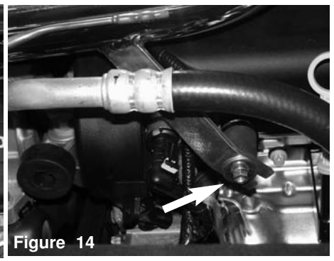
Figure 14 Align the intake bracket to the Vibramount from figure 10. Use a 10mm wrench and tighten the M6 nut and secure the bracket to the vibramount
