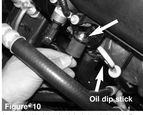
Figure 10 Locate the black bracket left of the oil dip stick. Place the Vibramount with a washer and M6 nut to secure it to the bracket
