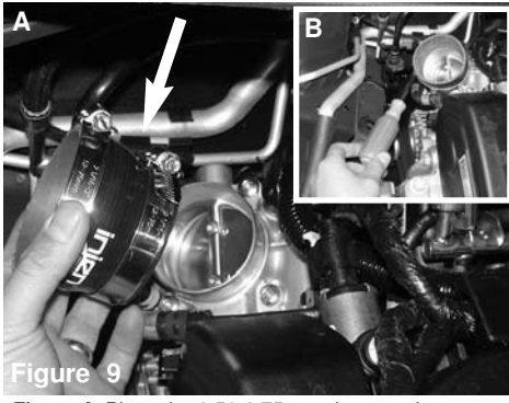
Figure 9 Figure A: Place the 2.50-2.75 step hose and two clamps onto the throttlebody. Figure B: Use a 8mm nut driver and tighten the clamp on the throttle body only for now.
