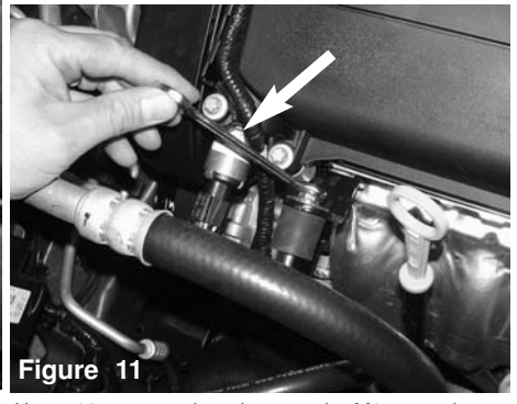
Figure 11 Use a 10mm wrench and secure the M6 nut to the Vibramount
