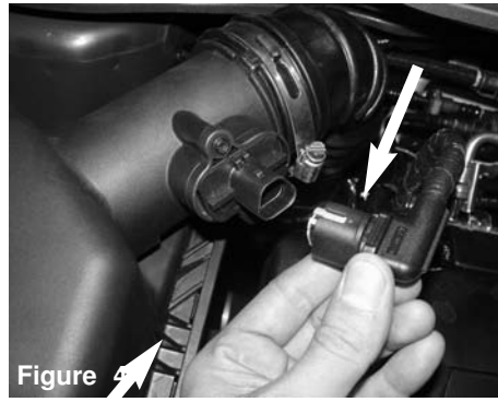
Figure 4 Disconnect MAF sensor harness.
