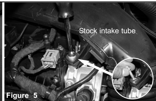
Figure 5 Locate the screw holding in the upper half of the stock intake tube. Loosen using 8mm nut driver or socket. Remove the screw.
