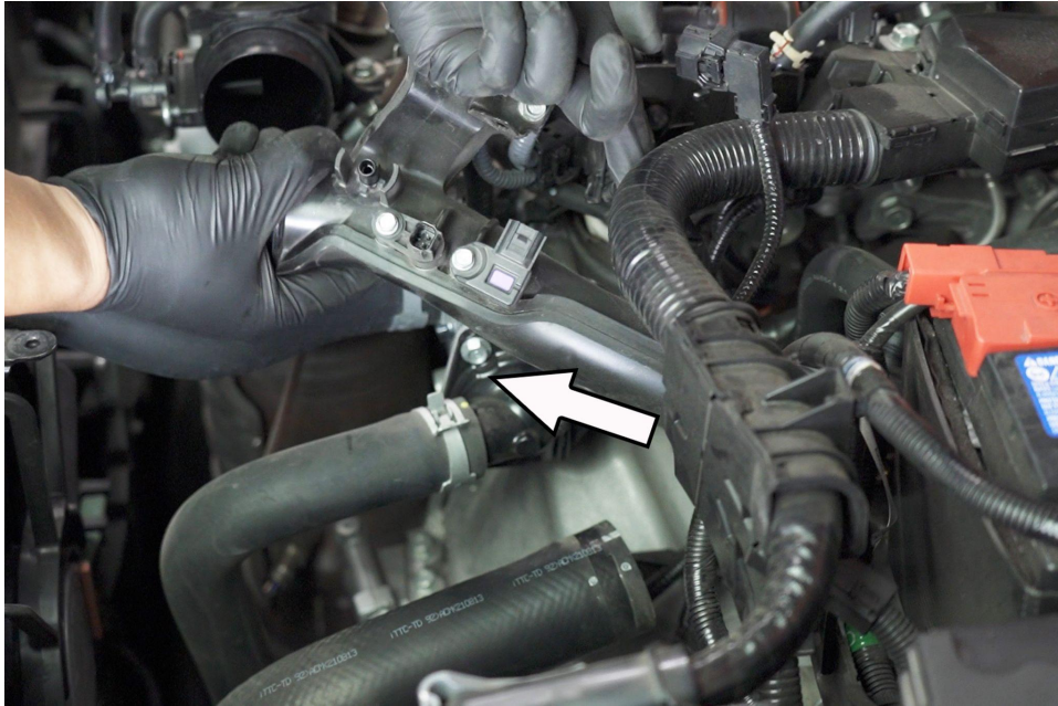
11. Carefully remove the factory charge pipe from the vehicle.
