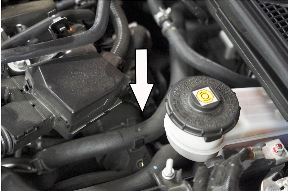
10. Loosen the hose clamp securing the charge pipe from the throttle body coupler. Disconnect the charge pipe from the coupler.
