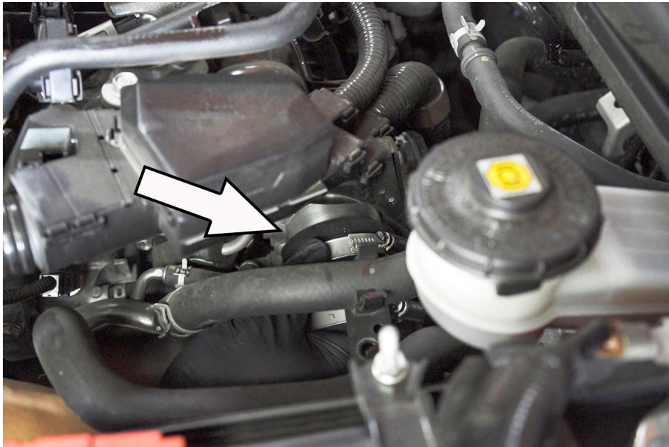
14. Insert the HPS straight coupler along with the two provided embossed clamps onto the throttle body. *Only secure the clamp on the side that's holding the coupler to the throttle body at this time.
