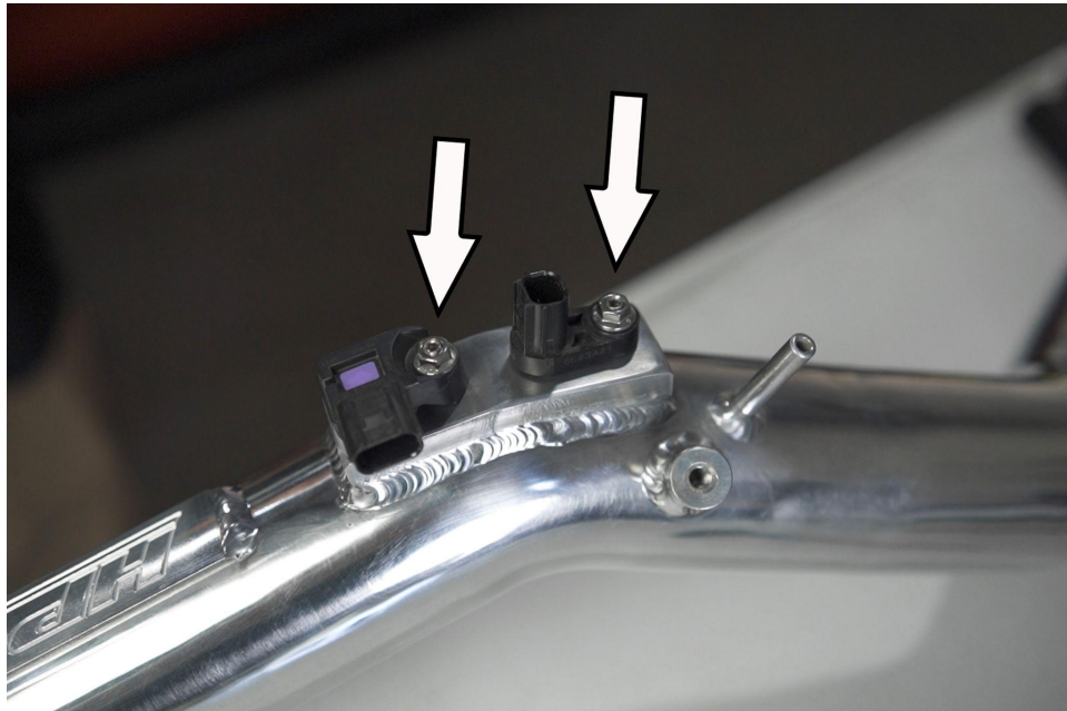
17. Secure the sensors using the two provided M5 nuts.
